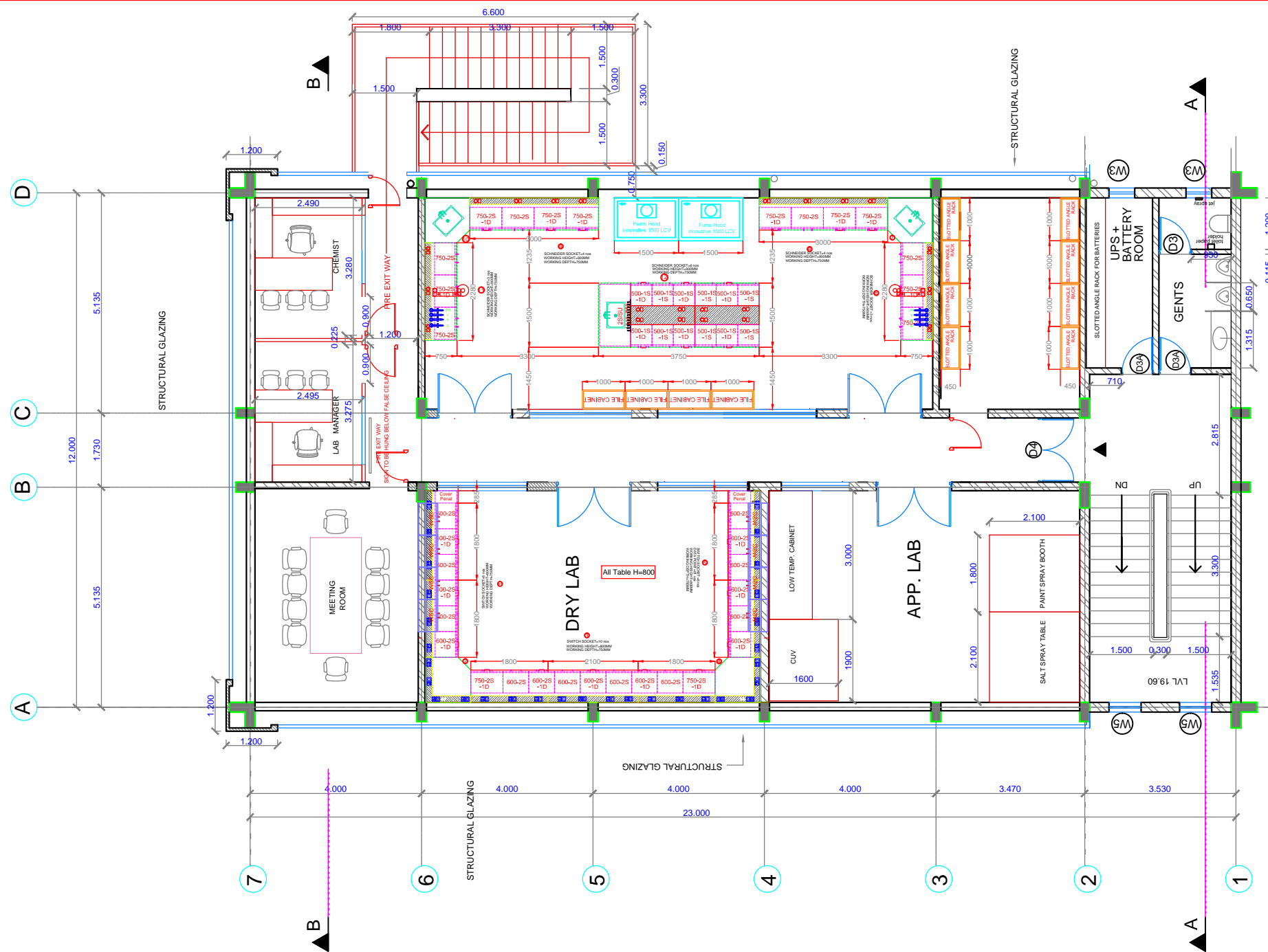
R&D LAB LAYOUT SECOND FLOOR PLAN
